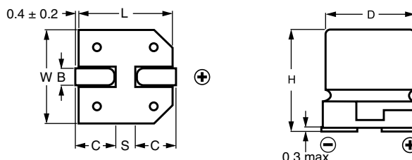
Fig.2 Dimensional outline
