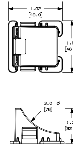
RTCM3EBL-L350
