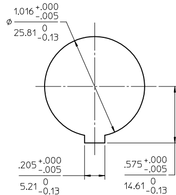
RECOMMENDED MOUNTING CUTOUT
