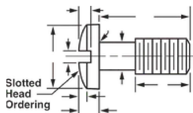
Slotted Head
